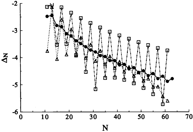
Figure 4. Convergence for a dielectric grating. ●, Sum of all diffraction efficiencies; □, diffraction efficiency of -1 order in reflection; Δ, diffraction efficiency of -1 order in transmission. The parameters are the same as for table 2.
