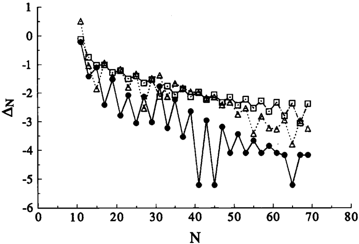
Figure 5. Convergence for a metallic grating. ●, Diffraction efficiency of -1 order; □, polarization angle \alpha ; Δ, polarization angle \delta . The parameters are the same as for table 3.
